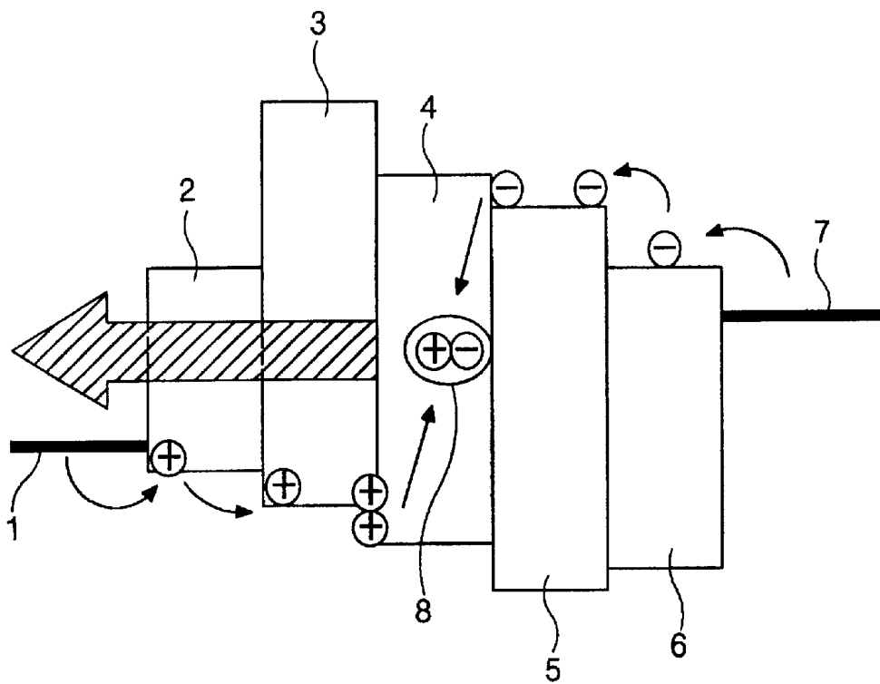
FIG. 1 (RELATED ART)
