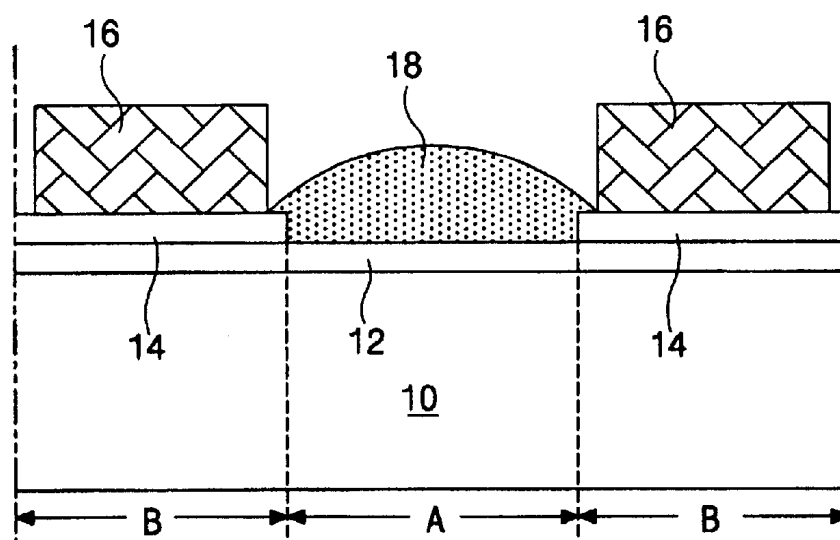
FIG. 2C (RELATED ART)
